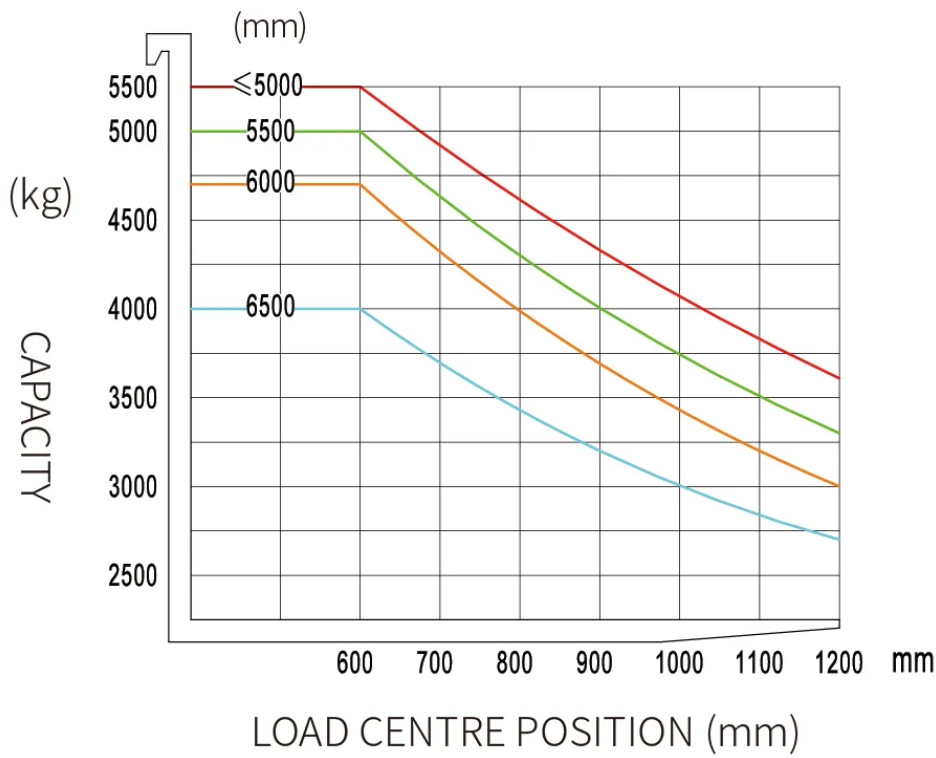
EFL553-HVD-6 RATED CAPACITIES AND LOAD CENTERES GRAPH
